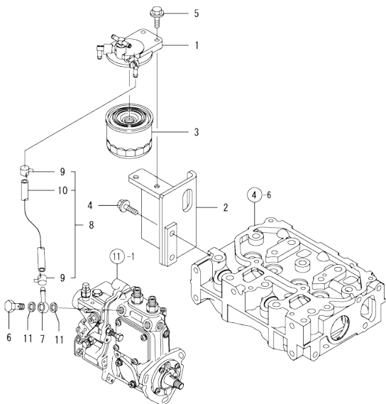
Fig.14. FUEL LINE
