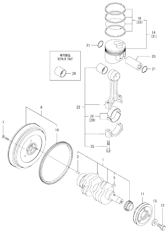
Fig.8. CRANKSHAFT & PISTON
